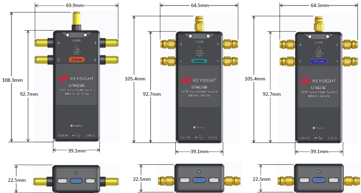
Figure 12. U9424x dimension (Option 002), SP4T
