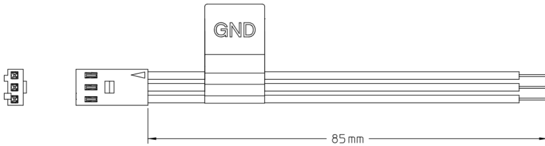
Figure 13. Option 101, 3-pins connector to bare wire, 85 mm (for SPDT Option 001 only) dimension
