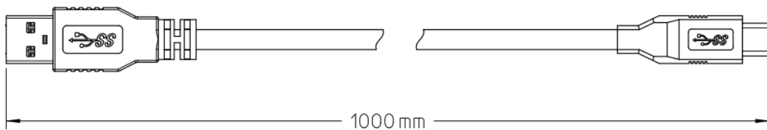
Figure 15. Option 201, USB 3.1 Type-A to Type-C, 1 meter (for Option 002 only) dimension
