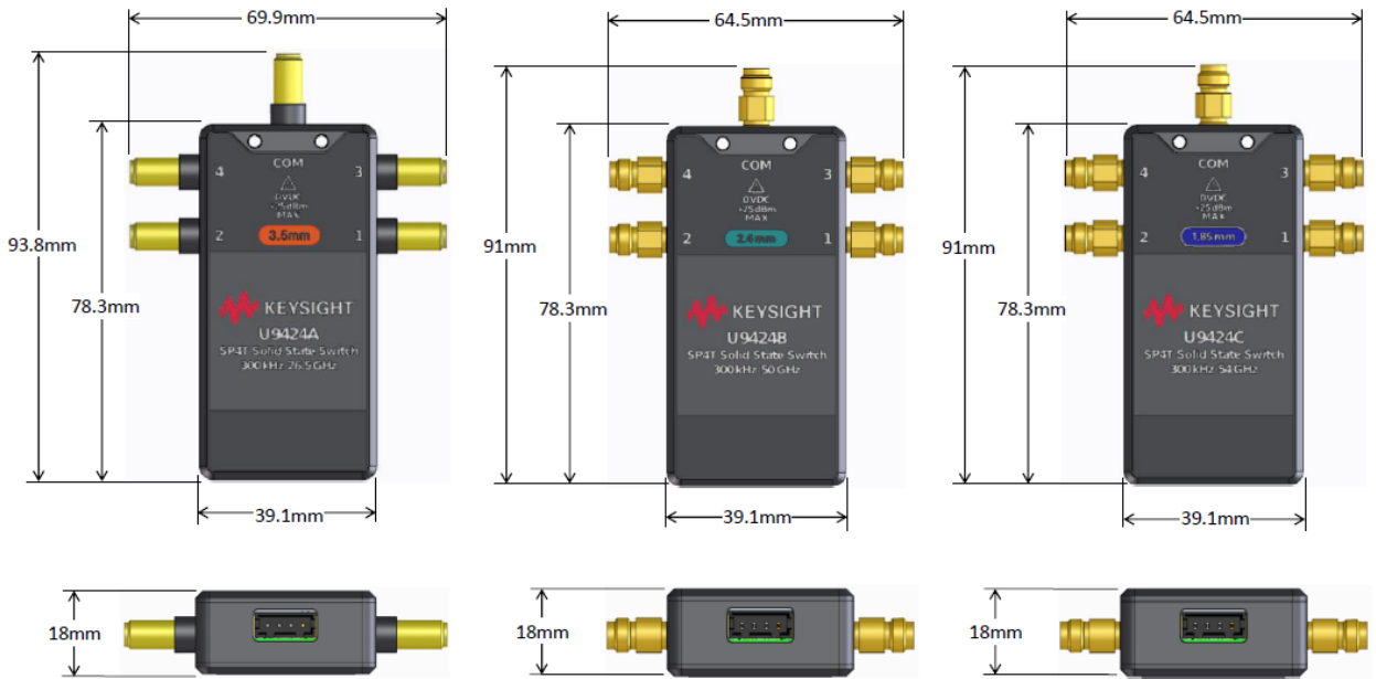
Figure 11. U9424x dimension (Option 001), SP4T
