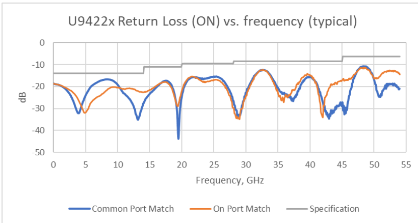
Figure 2. U9422x return loss (ON) vs frequency (GHz) typical
