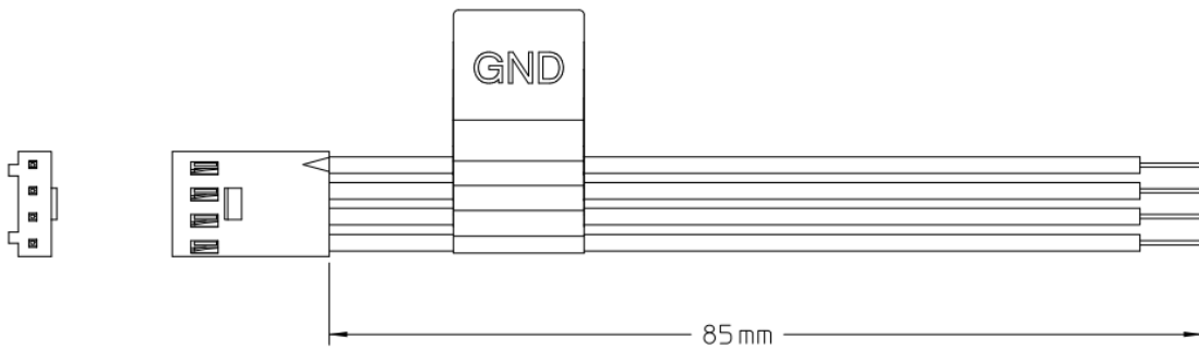
Figure 14. Option 101, 4-pins connector to bare wire, 85 mm (for SP4T Option 001 only) dimension
