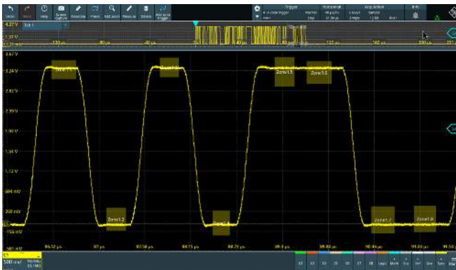
Use zone trigger on protocols to trigger on a specific packet sequence
