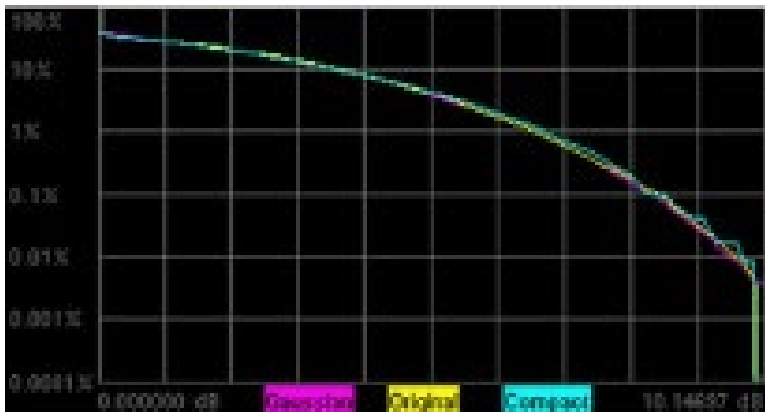
Figure 18. CCDF Comparison of the original 5G NR 100 MHz signal vs. compact test signal consisting of 10,001 tones. Share the same Power Spectral Density (PSD) and Complementary Cumulative Density Function (CCDF).
