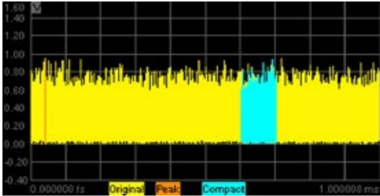
Figure 16. Example of a 5G NR 100 MHz parent-IQ waveform and Compact Tetra Signal (CTS) time slice
