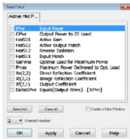
Hot S22 measurement with active parameter measurement function
