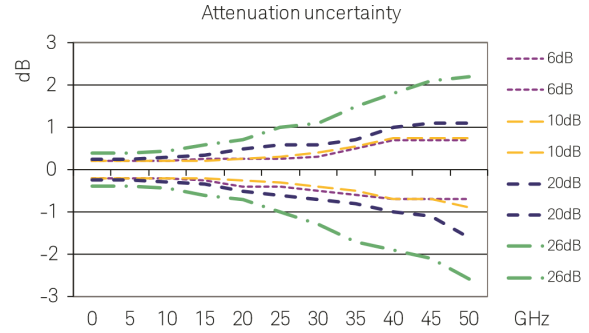
Figure 7. Attenuation Uncertainty (Characteristic)
