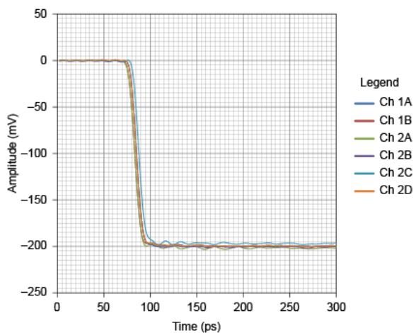
Figure 2. Options 52F, 52M, 54F, and 54M with TDR Calibration (Characteristic)
