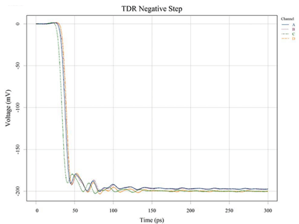
Figure 4. Options 52F, 52M, 54F, and 54M without TDR Calibration (Characteristic)
