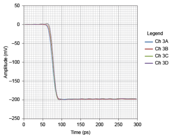
Figure 3. Options 32F, 32M, 34F, and 34M with TDR Calibration (Characteristic)
