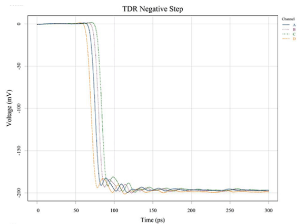
Figure 5. Options 32F, 32M, 34F, and 34M without TDR Calibration (Characteristic)
