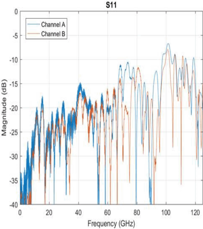
Figure 10. Graph of S11 ( characteristic )
