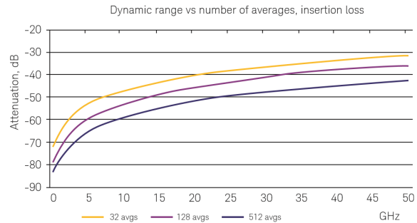
Figure 9. Dynamic Range vs Number of Averages, Insertion Loss (Characteristic)
