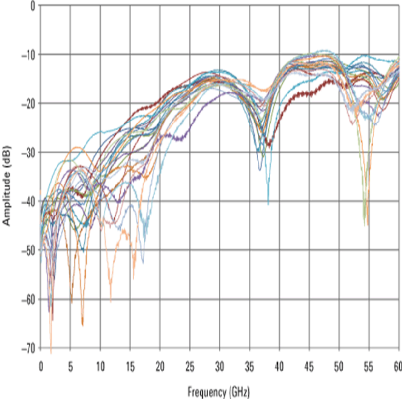
Figure 1. Graph of S11 ( characteristic )
