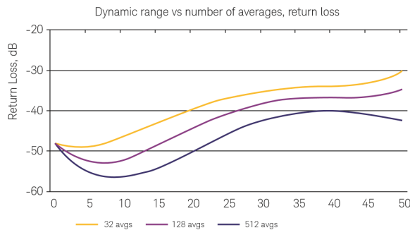
Figure 8. Dynamic Range vs Number of Averages, Return Loss (Characteristic)
