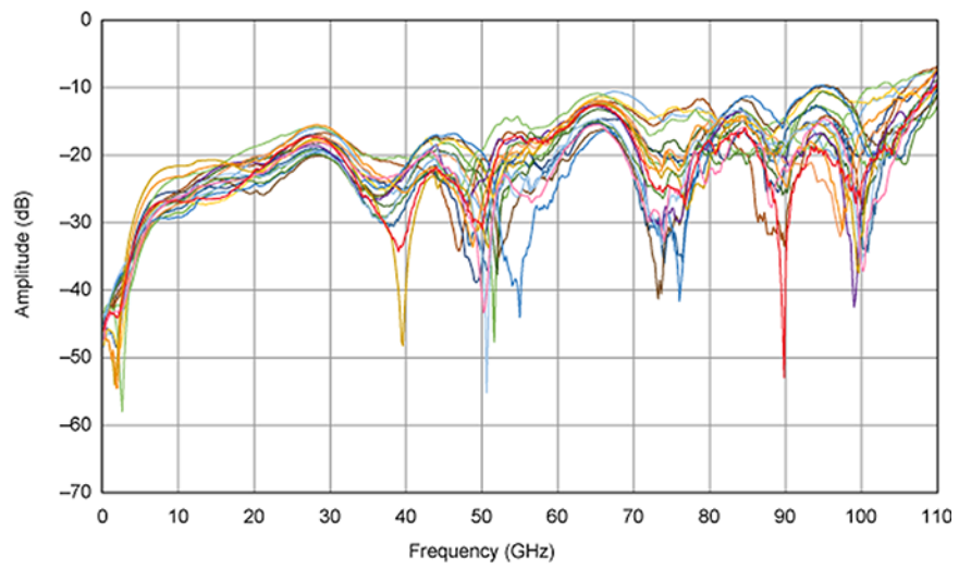
Input Impedance. Graph of S11 ( Characteristic )
