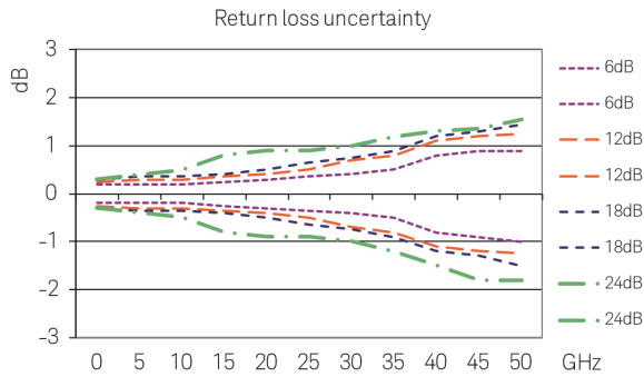
Figure 6. Return Loss Uncertainty (Characteristic)
