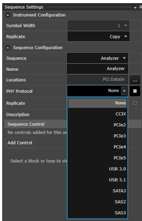
Figure 17. Users can select in the pattern sequencer menu between PCIe5, PCIe4, PCIe3, PCIe2, SAS 3, SAS 2, SATA 3, CCIX, USB 3.0 or USB 3.1 as PHY protocol to enable to the SKP OS and ALIGN filtering feature with M8046A-0S2 (PCIe), -0S4 (USB), or -0S6 (SATA/SAS)
