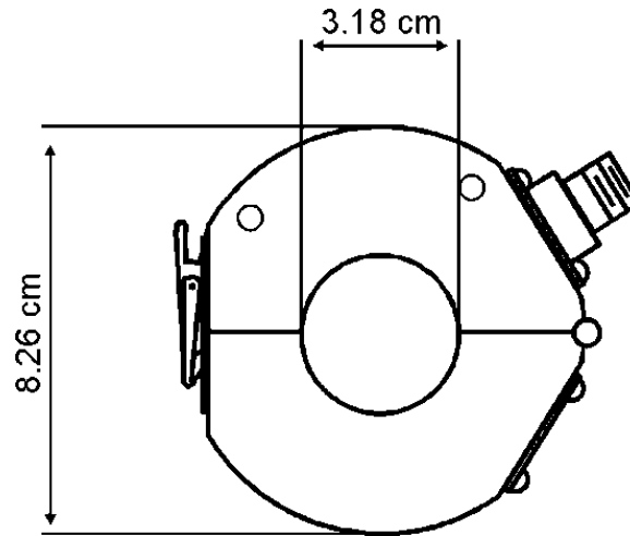
Model 93511 Series Current Probe
