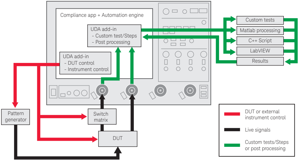
Figure 16: Combine the power of built-in automation and extensibility to transform your application into a complete test suite executable
