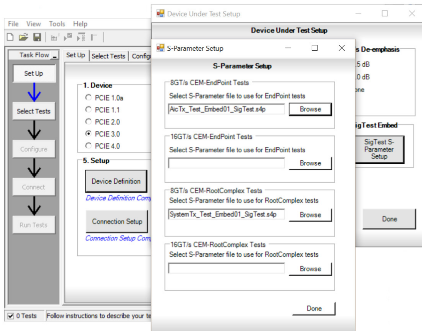
Figure 5: The D9040PCIC provides the option to use a user provided S-Parameter file S-Parameter file for 8 GT/s CEM testing
