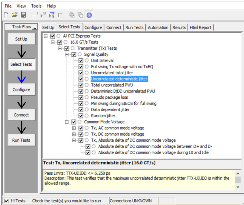
Figure 4: PCI Express 4.0 BASE Specification transmitter tests
