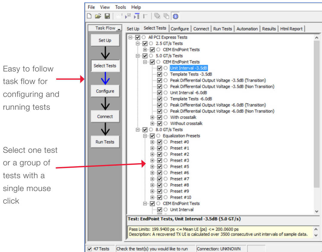
Figure 3: The Keysight automated test engine guides you quickly through selecting tests, configuring tests, setting up the connection, running the tests, and viewing the results. Individual tests or groups of tests are easily selected with a mouse click
