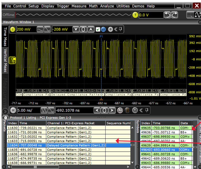
Figure 20: The N5463A provides 8b/10b and 128b/130b decode below
