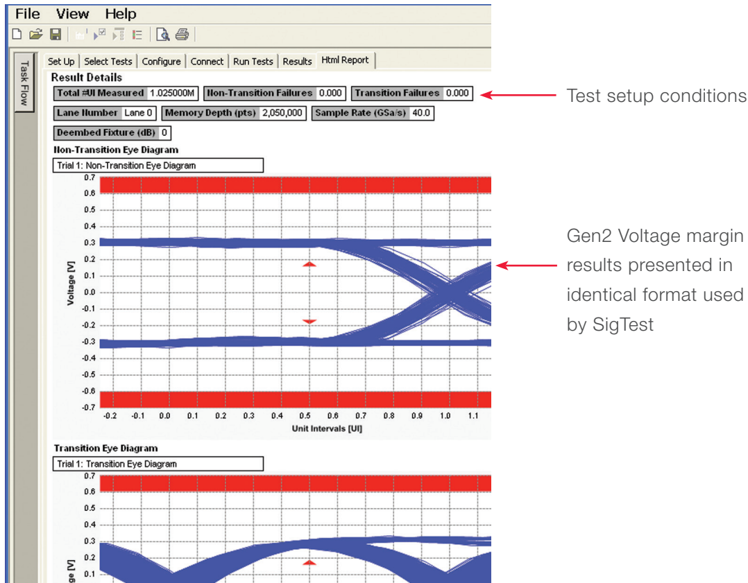
Figure 11: The HTML report provides additional details including test setup conditions, graphical results, and test limits (where appropriate)
