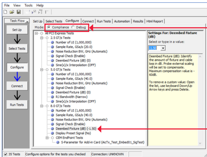
Figure 7: In the Configure tab you can set parameters like number of UI, noise reduction, signal check, etc.
