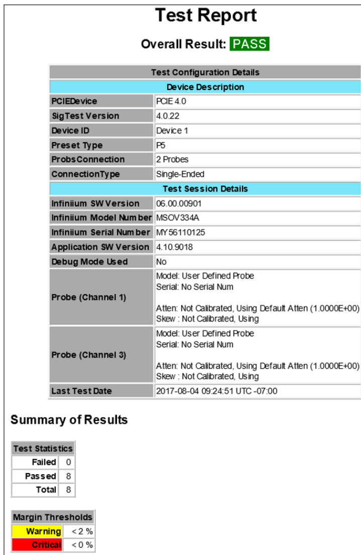
Figure 10: The PCI Express electrical test software results report documents your test, indicates the pass/fail status, the test specification range, the measured values, and shows how much margin you have
