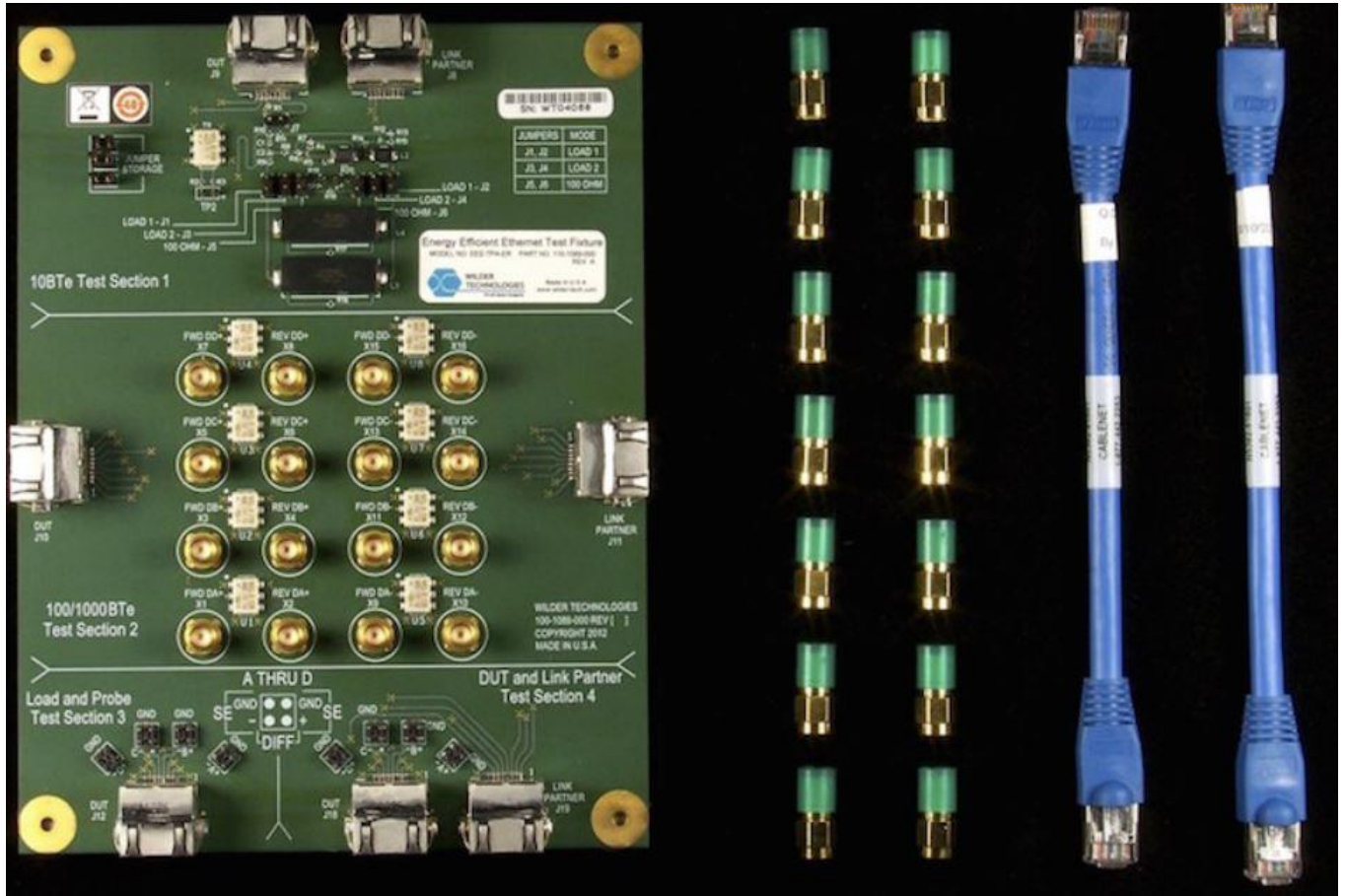
Figure 8. The EEE-TPA-ERK Wilder Technologies Energy Efficient Ethernet test fixture allows you to test to the 10BASE-T e , 100BASE-T Xe and 1000BASE-T e Energy Efficient Ethernet standards. Sold separately through Wilder-Technologies.
