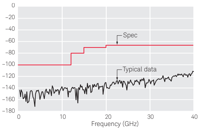
Figure 12. 87104/6D isolation loss versus frequency
