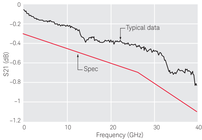
Figure 11. 87104/6D insertion loss versus frequency
