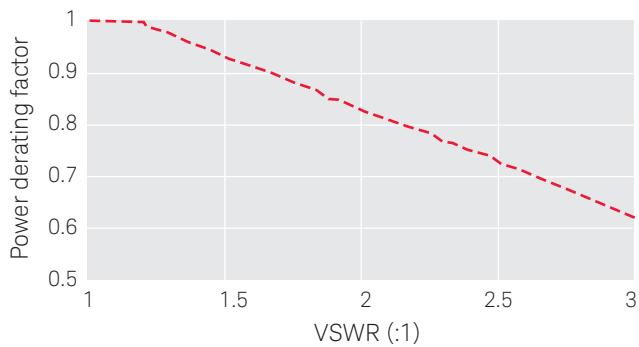
Figure 9. Power derating factor versus VSWR
