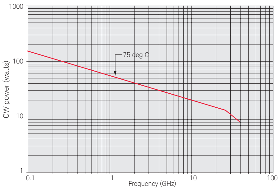
Figure 8. Maximum incident CW power (cold switching) vs. frequency
