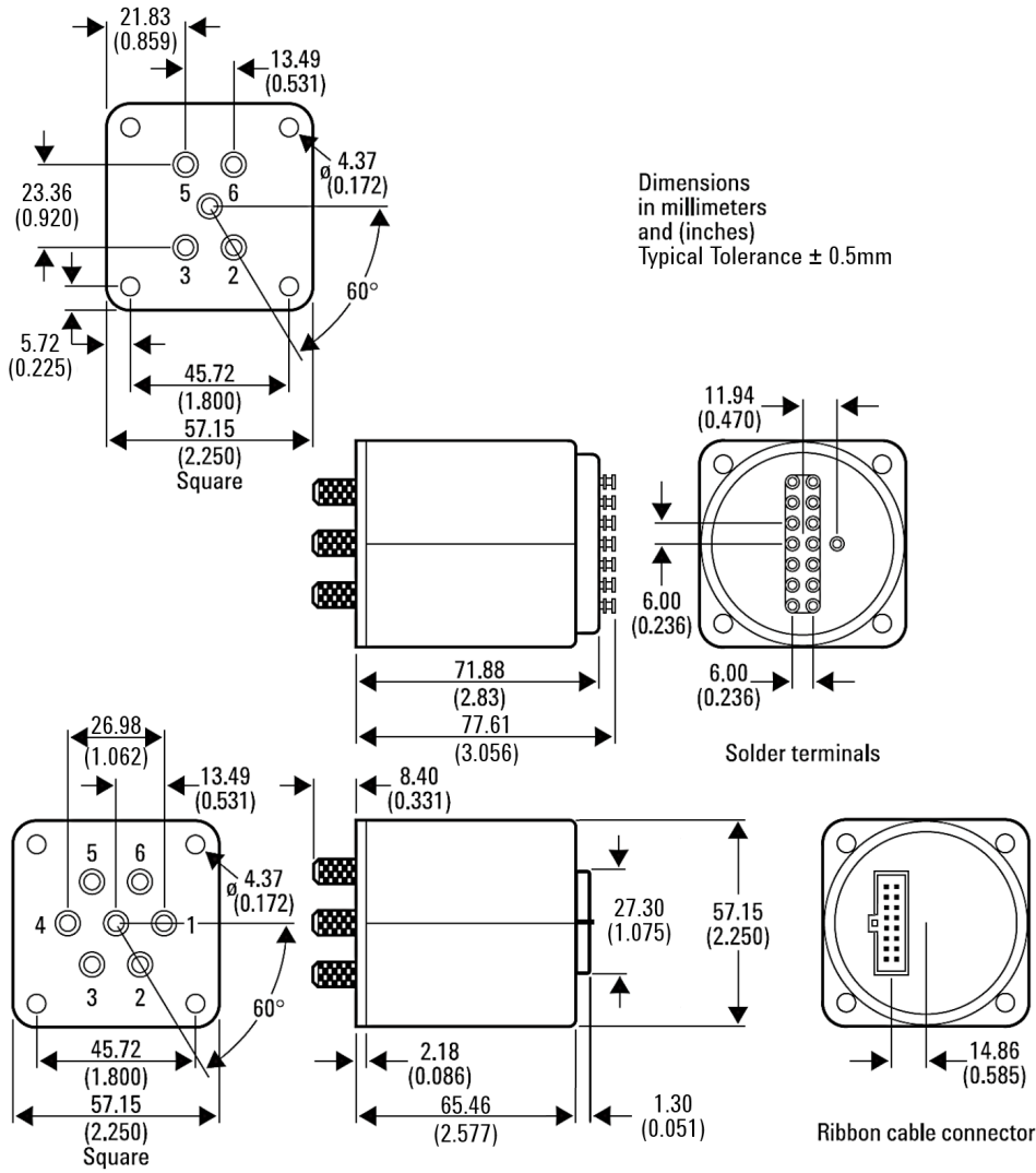
Figure 13. Mechanical dimensions
