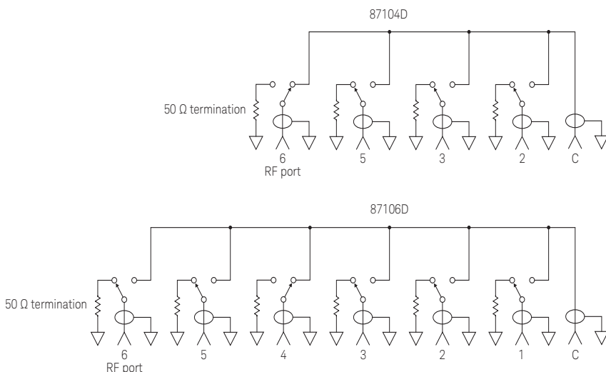
Figure 2. Keysight 87104D and 87106D simplified schematics
