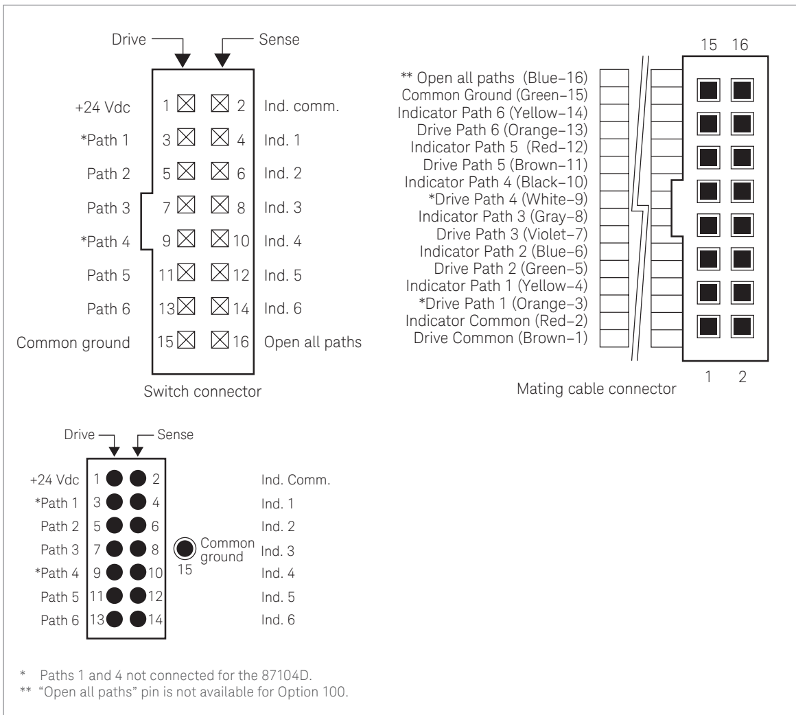
Figure 14. Drive connection diagrams with Option 100
